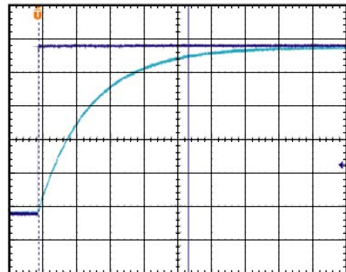
Figure 21. Turn-On Time— C_x, C_y = 0.1 \mu\text{F} , Time Scale = 2 ms/DIV
